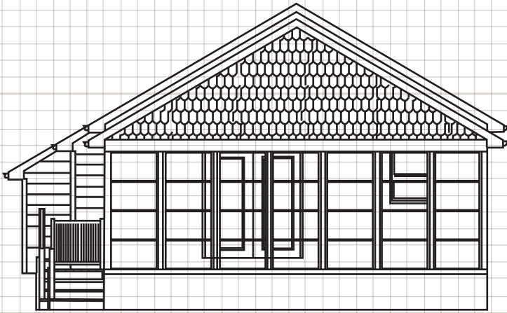
FRONT ELEVATION .....
